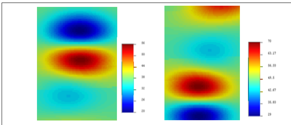
Figure 7. Map of distribution of downy mildew on var. P35 (Sumbergirang 2) at week 5 (left) and week 10 (right)
