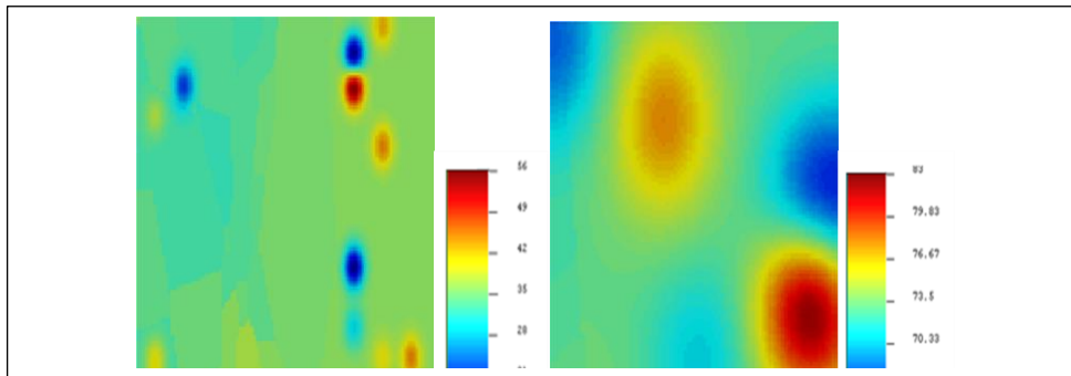
Figure 6. Map of distribution of downy mildew on var. NK 6172 Sumbergirang 1 at week 5 (left) and week 10 (right)
