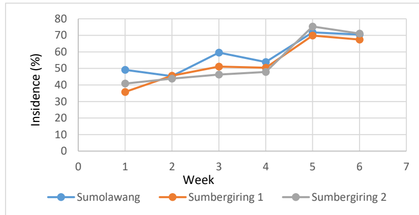
Figure 3. Development of downy mildew at several study
