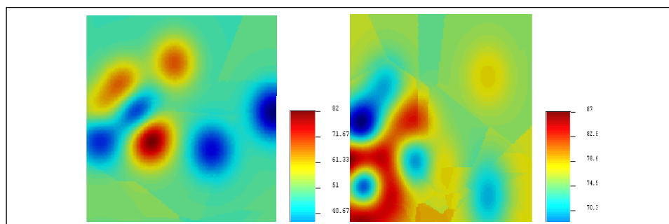
Figure 5. Map of disease distribution in corn var. NK 6172 (Sumolawang) at week 5 (left) and week 10 (right)
